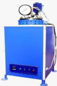
CEMENT AUTOCLAVE
